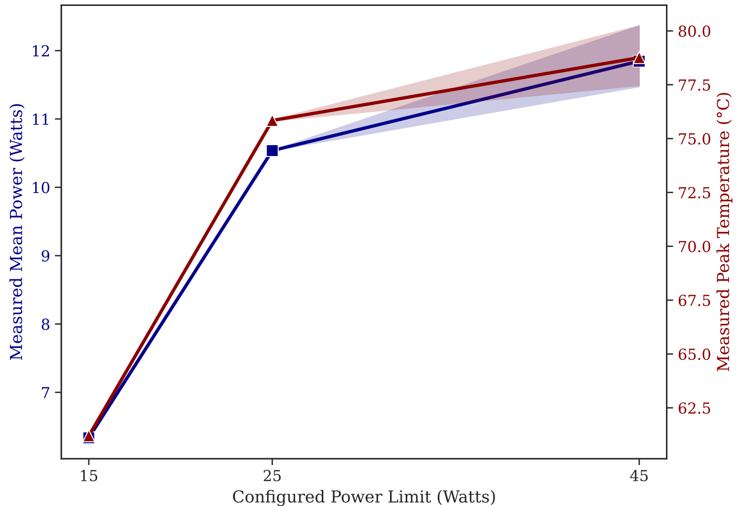
Figure 2: Hardware Validation of Power-Thermal Throttling
